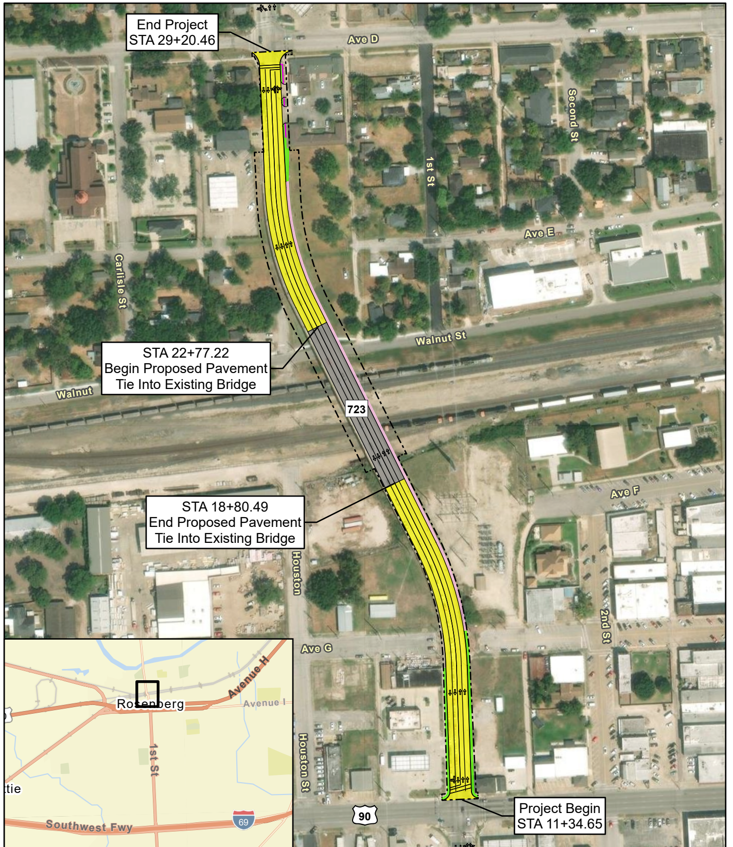
Figure 1. Schematic Layout
